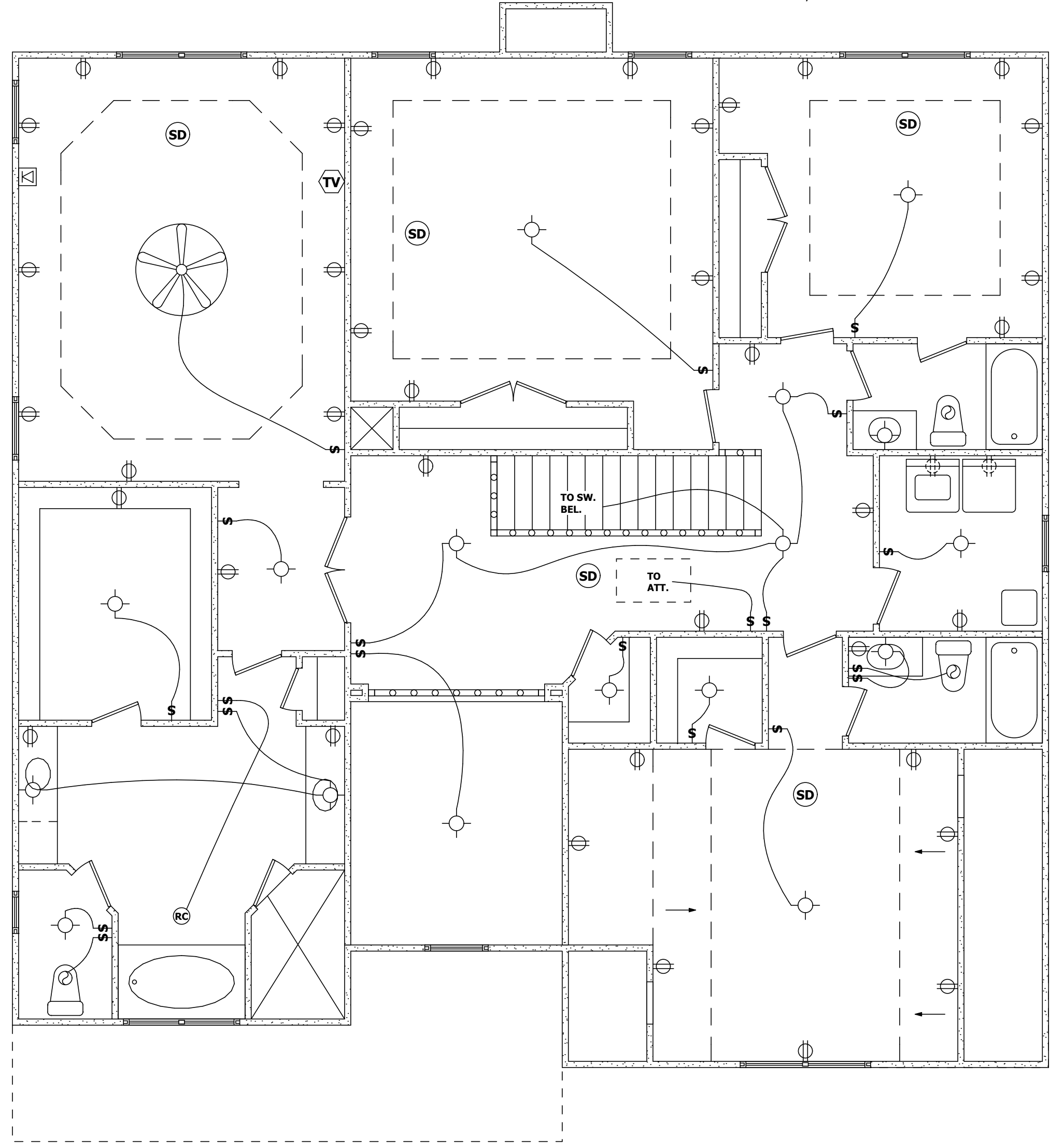
SECOND FLOOR ELECT. PLAN N.T.S.
