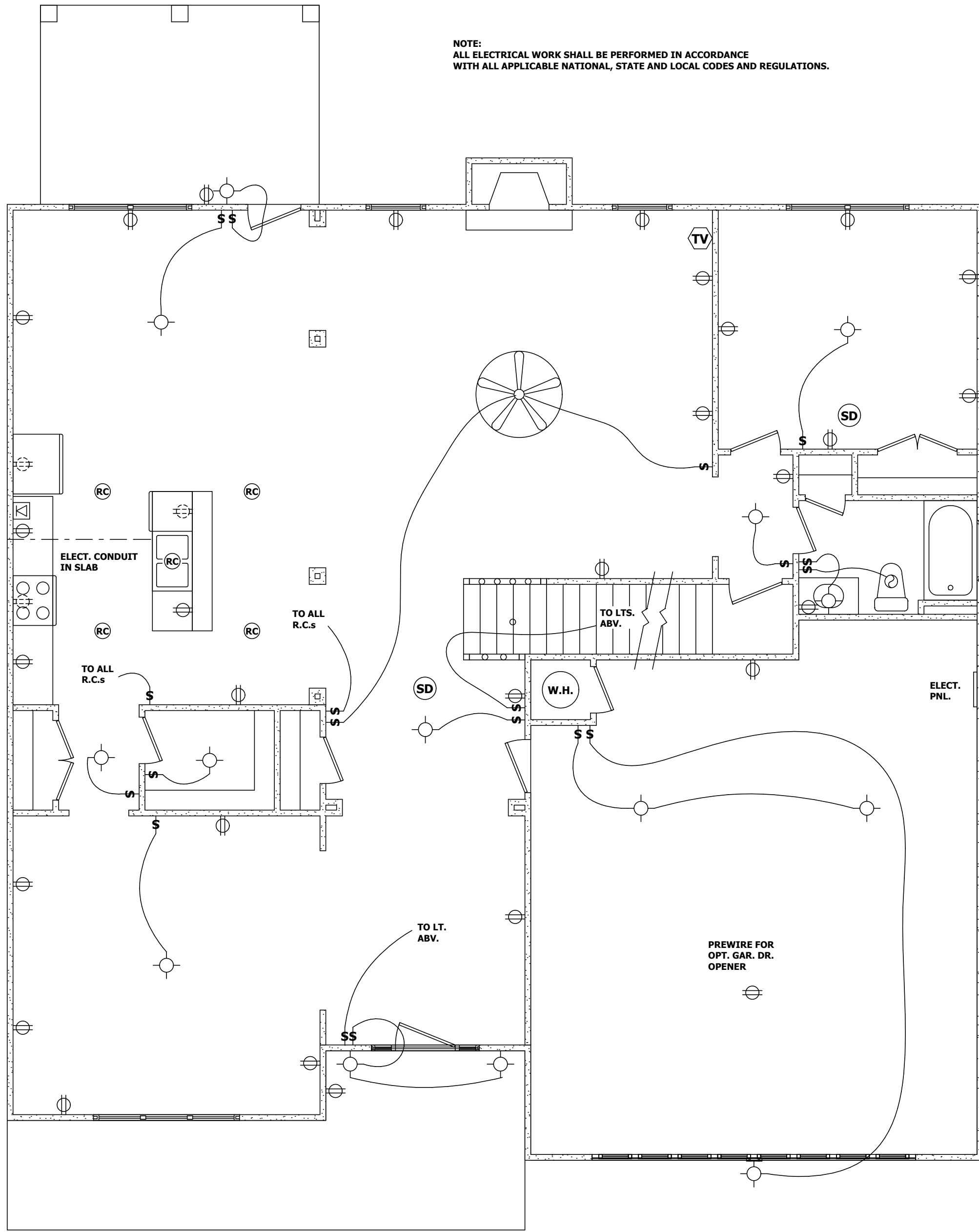
FIRST FLOOR ELECT. PLAN N.T.S.
