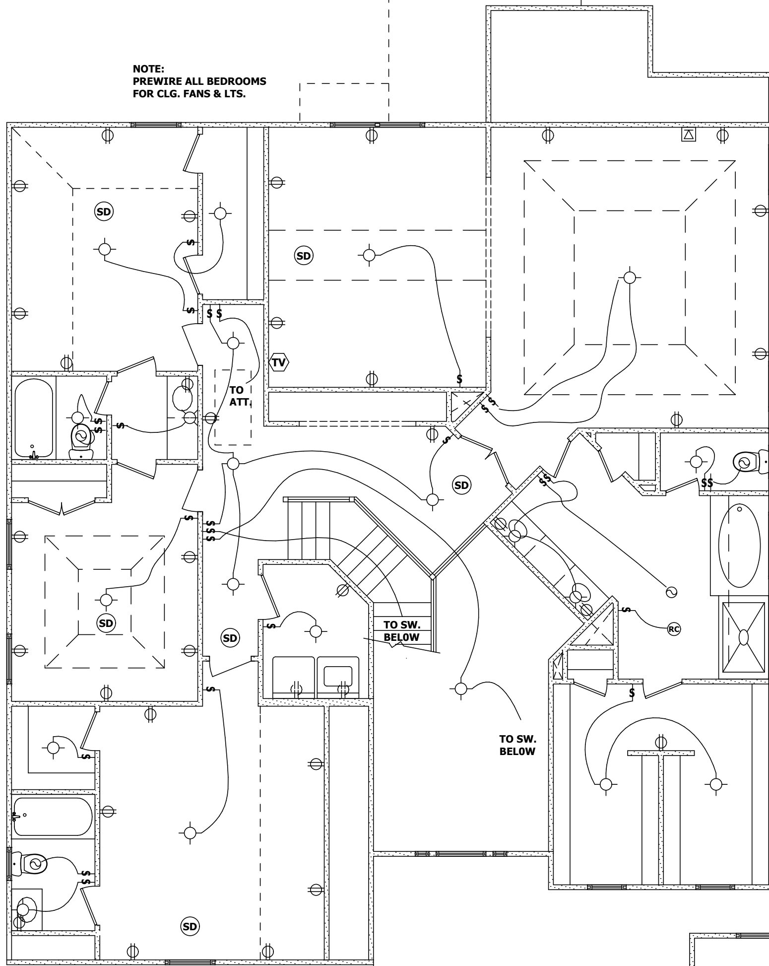
SECOND FLOOR ELECT. PLAN N.T.S.
